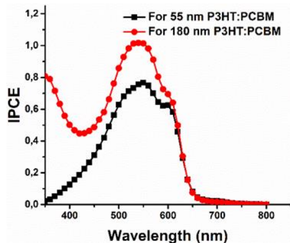
Fig. 5. IPCE values of P3HT:PCBM blend various thicknesses with 5 nm Ca thickness at wavelengths
